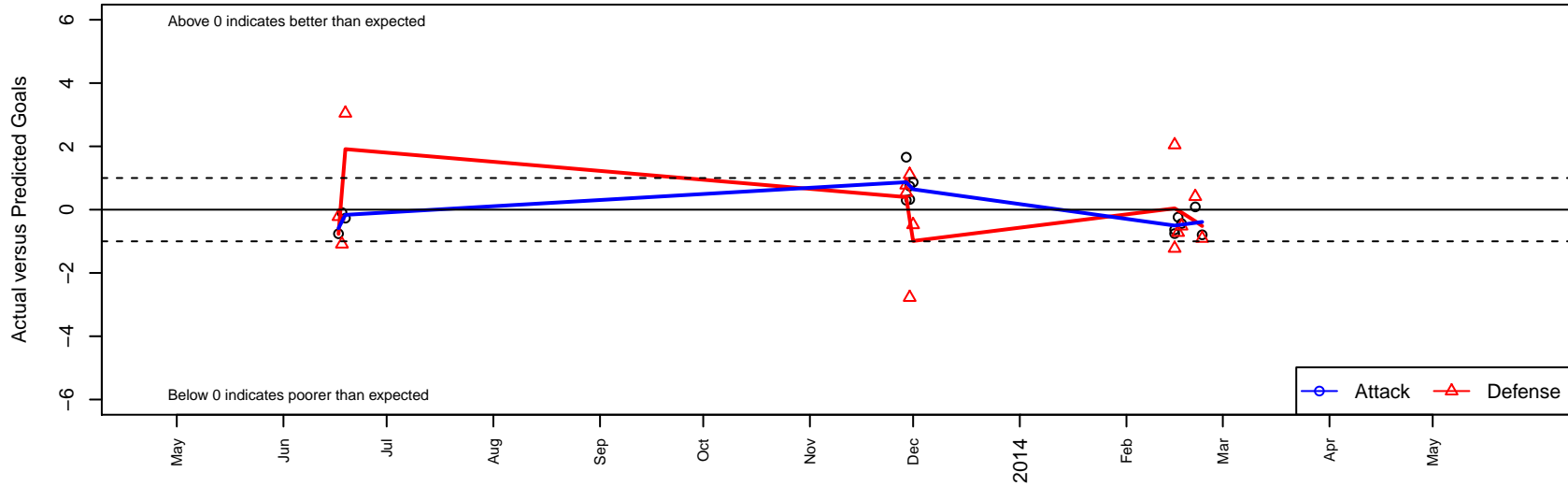
San Tan SC 00 Legacy Red G99 Dots are actual minus expected GF (blue circles) and GA (red triangles). Blue line is smoothed change in attack strength. Red is smoothed change in defense strength.
